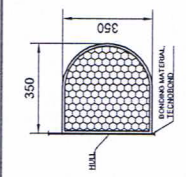
SECTION FENDER, D-TYPE
